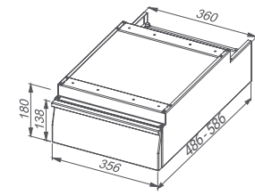
Single drawer: plain/frame for GN 1/1 container
