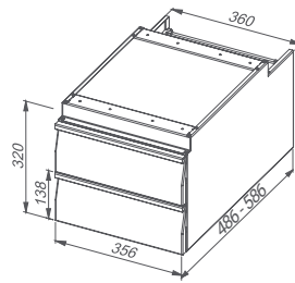
Double drawer block: plain/frame for GN 1/1 container
