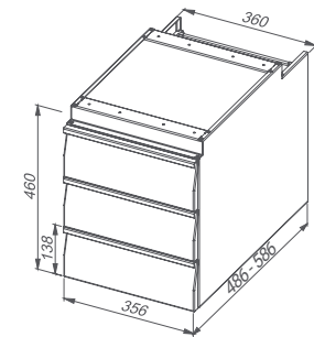
Triple drawer block: plain/frame for GN 1/1 container
